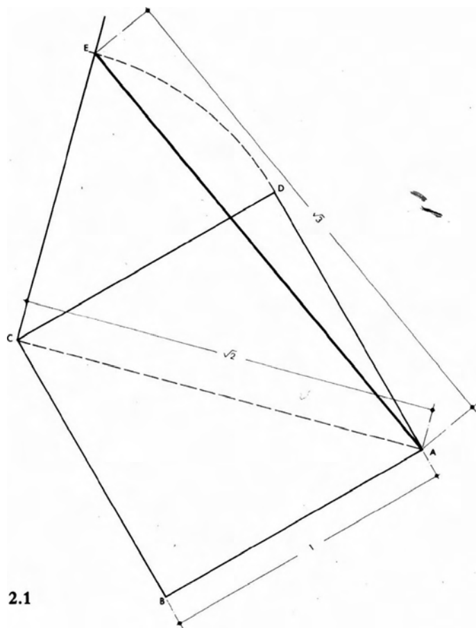
Drawing 2.1. Draw square ABCD (it is shown here at a 30^\circ angle so as to be visually comparable
