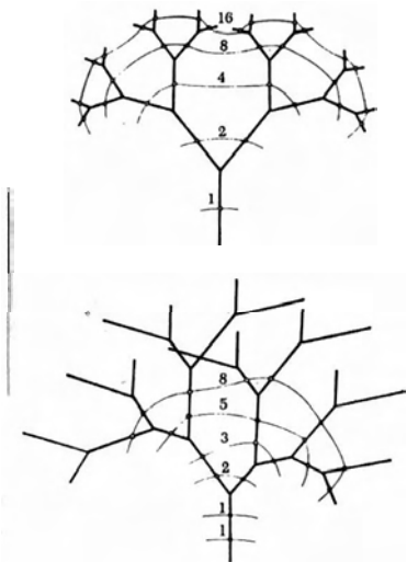
The two major branching patterns, one demonstrating the geometric progression by 2(\sqrt{2}) , and the other the Fibonacci Series (4).
