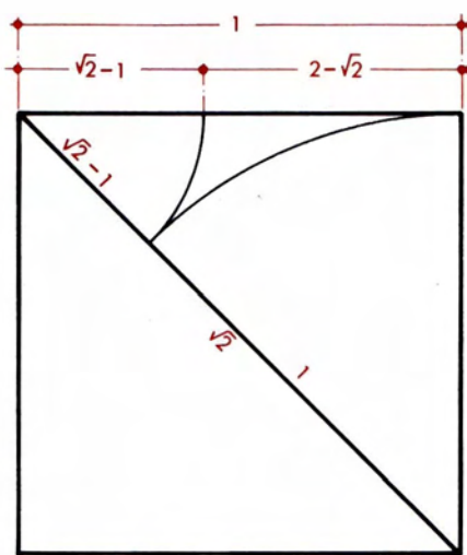
Drawing 8.2. (\sqrt{2}-1):(2-\sqrt{2}):1 Harmonic
