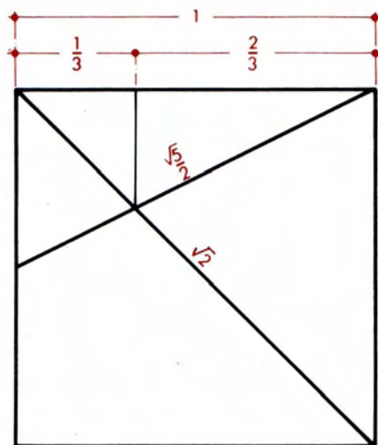
Drawing 8.1. \frac{1}{3}:\frac{2}{3}:1 Arithmetic
