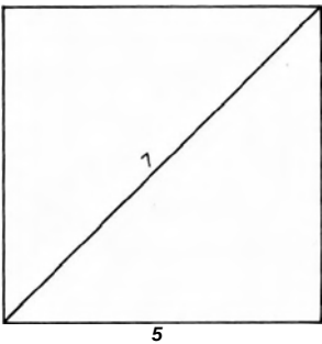
SQUARE A-3 diag = 7 side = 5
